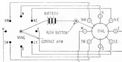
The wiring diagram showing the electrical connections between the vane and the dial
